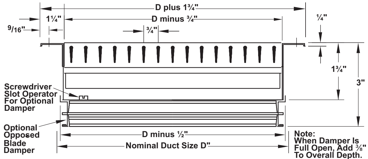
Double Deflection Models 300RL / RS - Border Type 1
