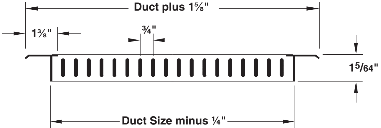
Single Deflection Models 301RL-SS / RS-SS - Border Type 1
