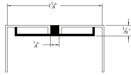
DETAIL B-B
