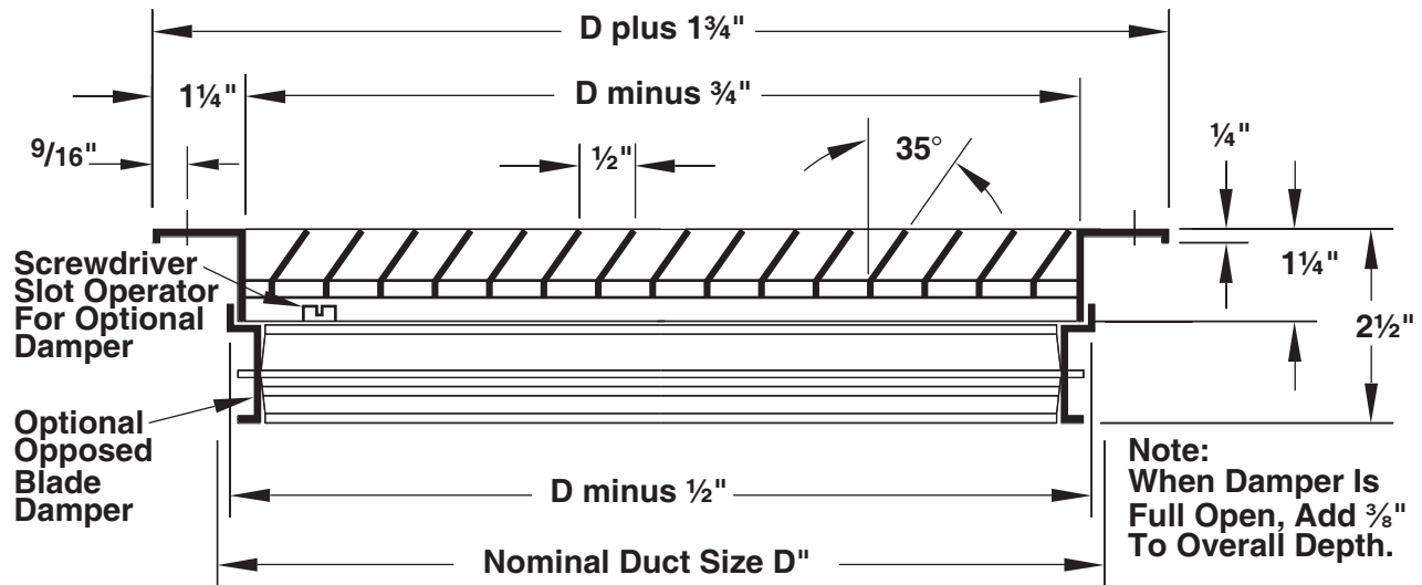
35° Deflection Models: 355RL / 355RS - Border Type 1
