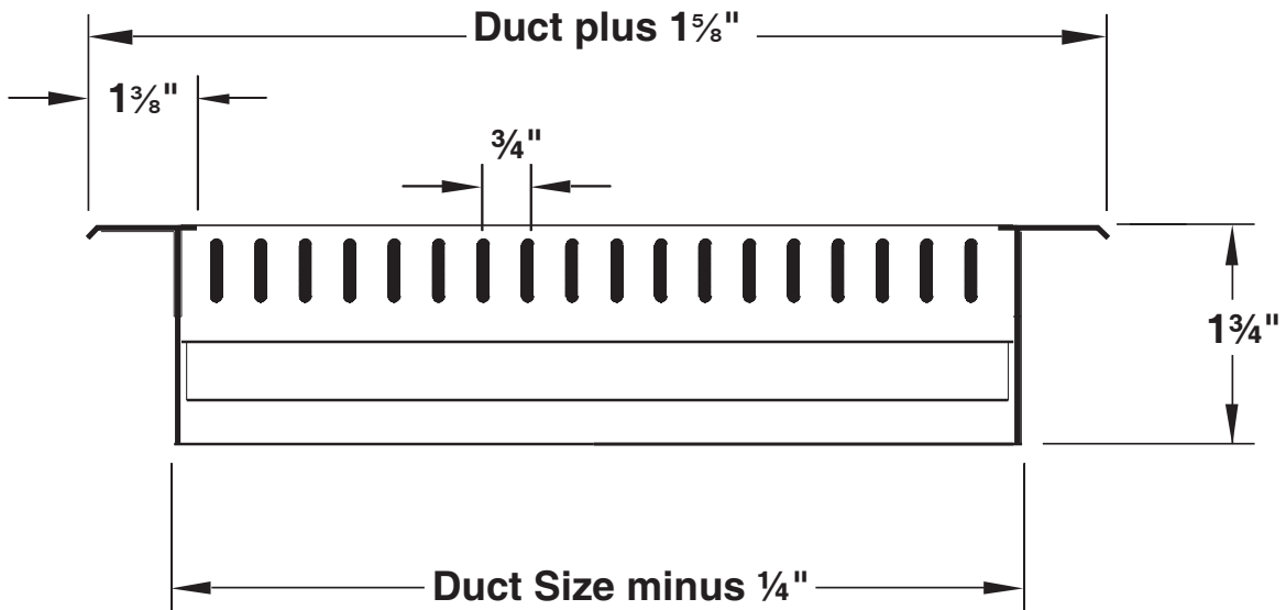
Double Deflection Models 300RL-SS / RS-SS - Border Type 1
