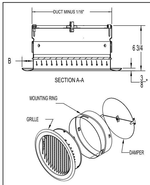
Damper option
