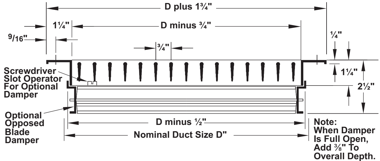
Single Deflection Models 301RL / RS - Border Type 1
