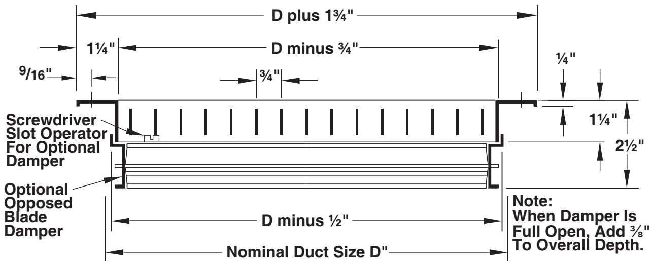
0° Deflection Models: 350ZFL / 350ZFS - Border Type 1
