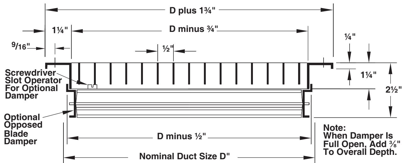
0° Deflection Models: 355ZRL / 355ZRS - Border Type 1
